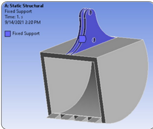
Fix Support Point of Excavator Claw
