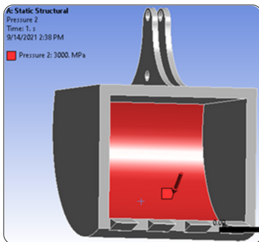
Pressure Area of Excavator
