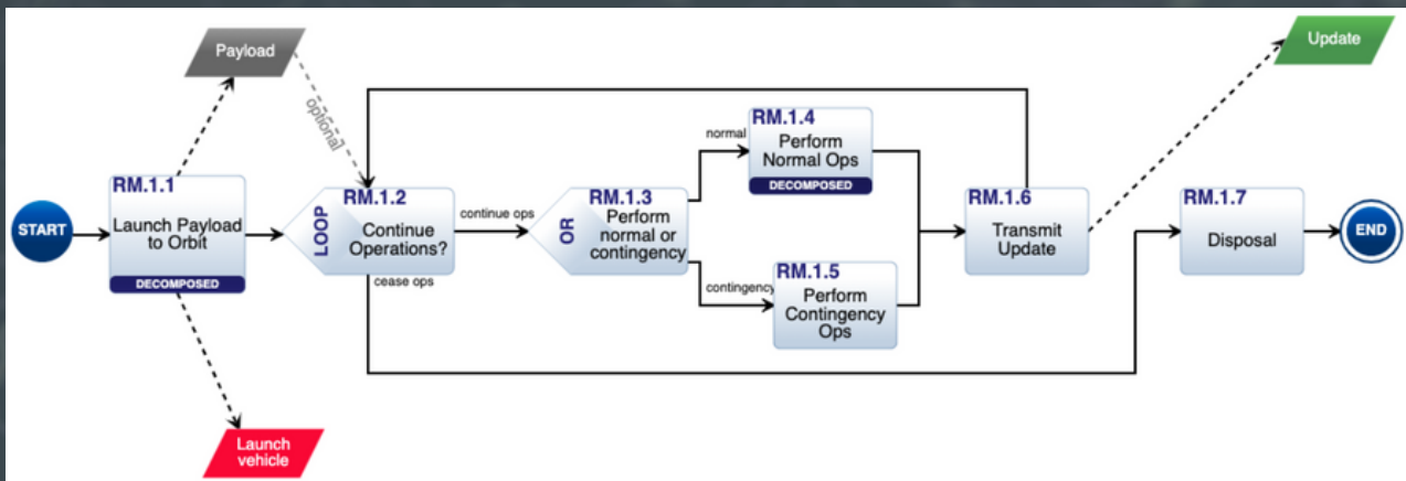
LML Action Diagram Example
