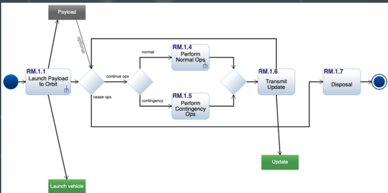
SysML Activity Diagram
