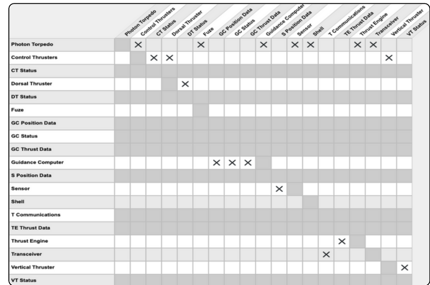
Figure 26. Lesson 10 in Innoslate
