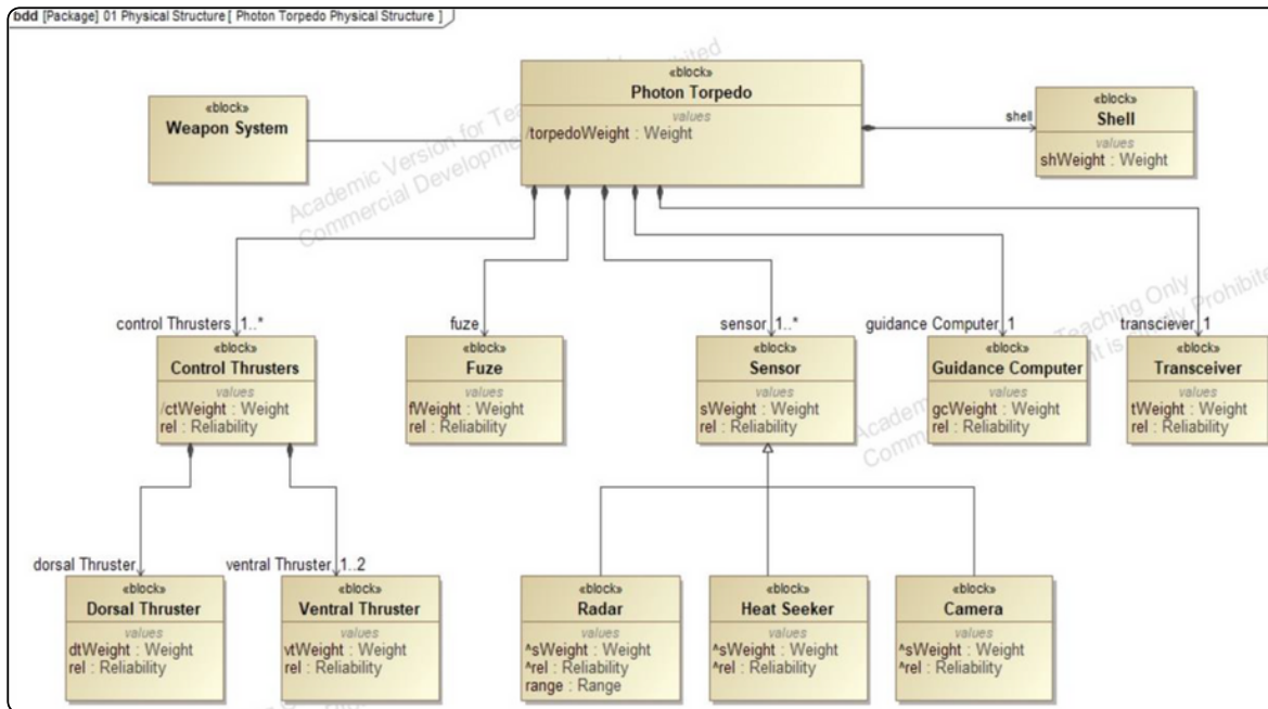
Figure 13. Lesson 4 in Cameo
